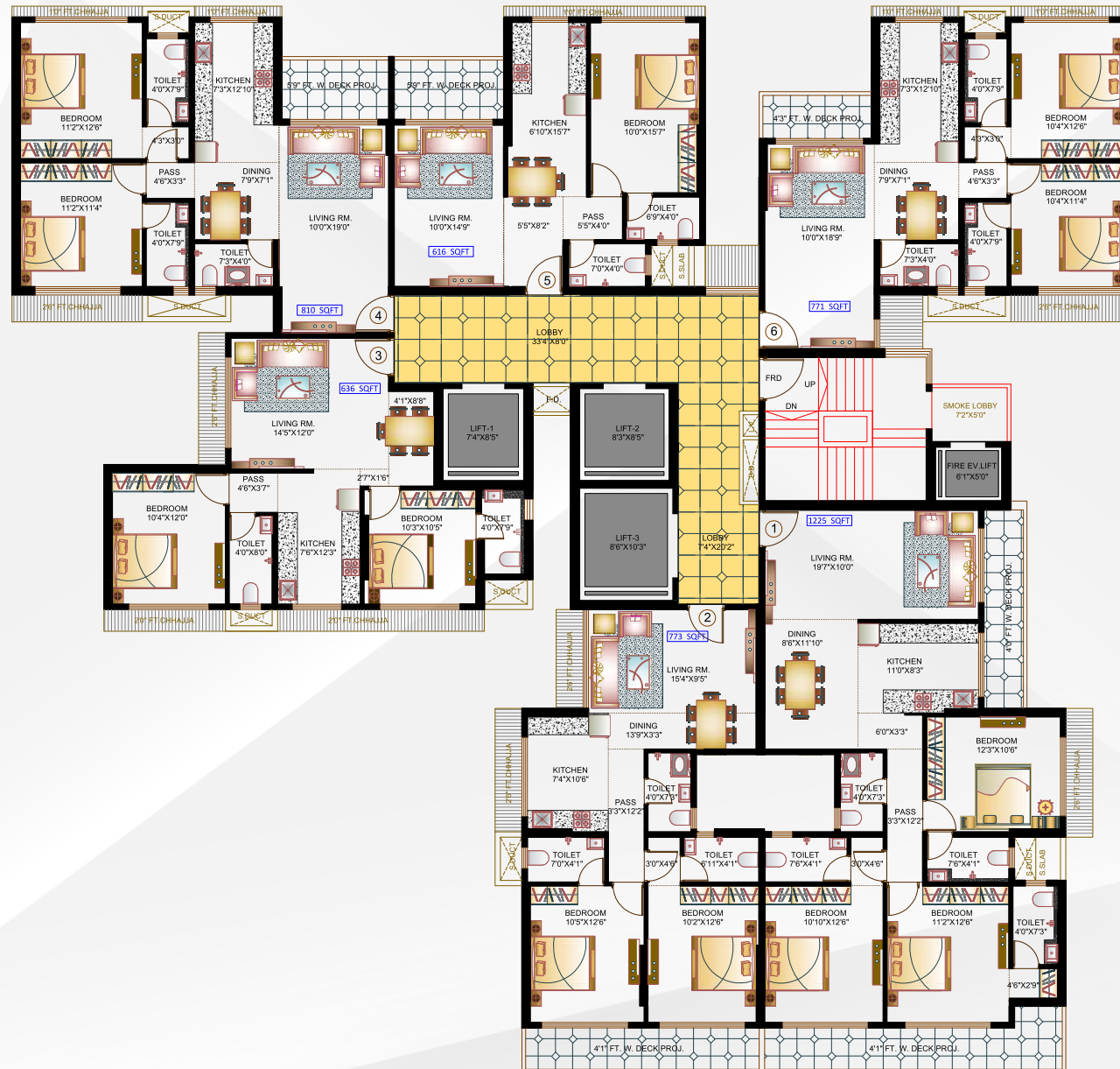
19 th & 20 th FLOOR PLAN
